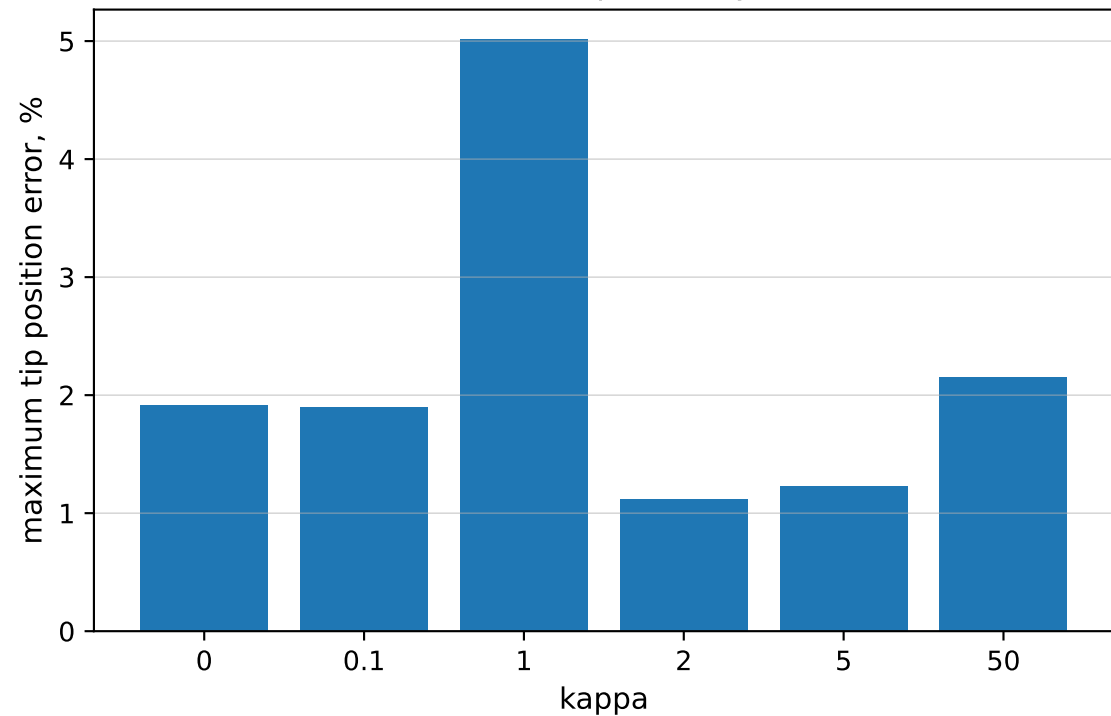
Maximum PRB 3R Tip Error by Load Ratio
